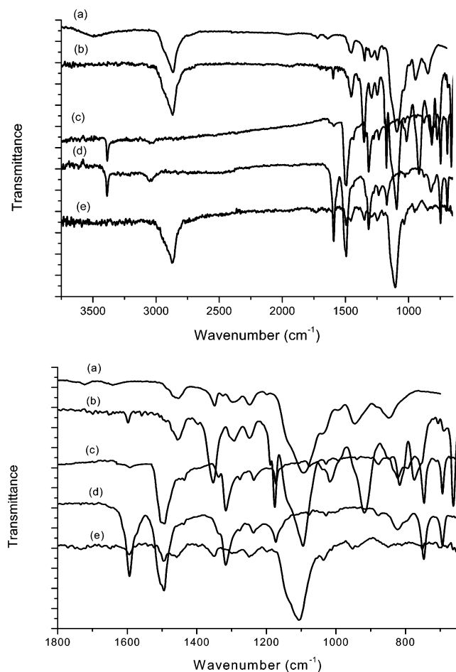
Figure 1. FTIR spectra of PEO-2000, PEO-Tos-2000, neutralized PDPA, reduced PDPA, and neutralized PDPA- g -PEO-2000: (a) PEO-2000, (b) PEO-Tos-2000, (c) reduced PDPA, (d) neutralized PDPA, and (e) neutralized PDPA- g -PEO-2000.
