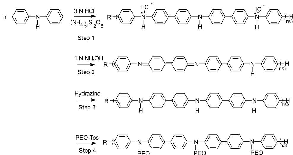
Scheme 1. Synthesis Strategy of Polydiphenylamine Grafted with Poly(ethylene oxide) (PDPA- g -PEO) through a "Graft Onto" Process
